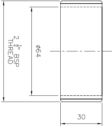
(SCALE-1:4) DETAIL-A BUSH FOR COUPLER
